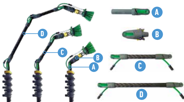
nLite® Connect WINKELADAPTER ELEMENTE
